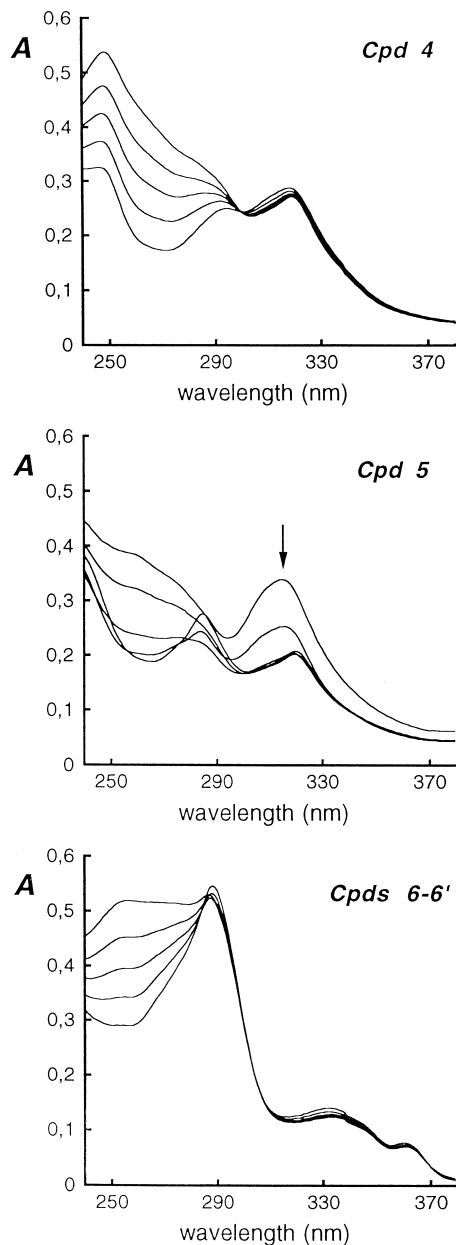
Figure 3. Absorption spectra of compounds 4 , 5 , and 6–6' in the absence and presence of calf thymus DNA. To 3 mL of drug solution (10 \mu M in 10 mM Tris, 10 mM NaCl buffer, pH 7.1) were added successive amounts of DNA. The DNA/drug ratio increased as follows (bottom to top curves at 260 nm): 0, 1, 2, 3, and 4. With compound 5 , at higher P/D (phosphate–DNA/drug) ratios no further qualitative changes occurred and the hypochromism at 320 nm plateaued at about 40%.
